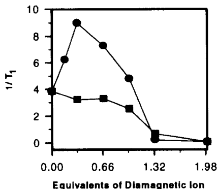
Figure 2. Effect on the observed ^{31}\text{P} relaxation rate of diethyl p -methoxyphenyl phosphate as a function of increasing diamagnetic ion concentration: \text{Zn}^{2+} (●) and \text{Cd}^{2+} (■).
